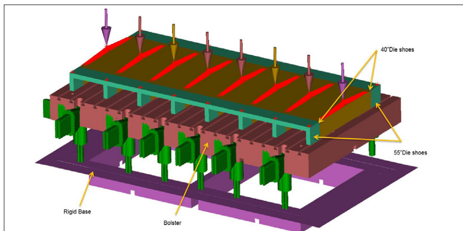
Figure 1: 1000-ton press die bolster model
