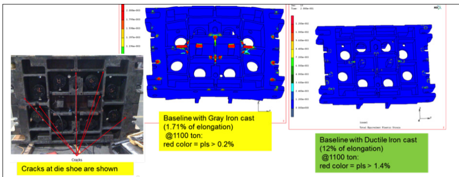
Figure 3: Total equivalent plastic strain plot of gray cast iron die shoe matches cracks seen in the physical die shoe while simulation of the ductile cast iron shoe indicates that cracking will not occur.
