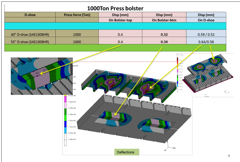
Figure 2: Results of the die bolster study show that the die bolster deflection is less than the die shoe
