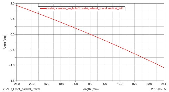
Camber vs wheel travel
