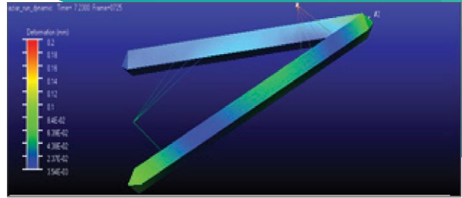
Deformation after dynamic suspension analysis
