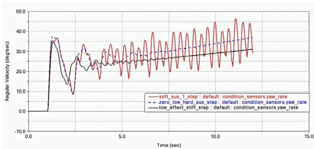
Yaw rate vs time
