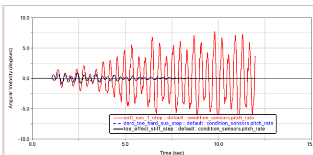
Pitch rate vs time
