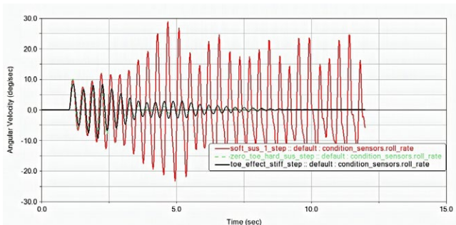
Roll rate vs time
