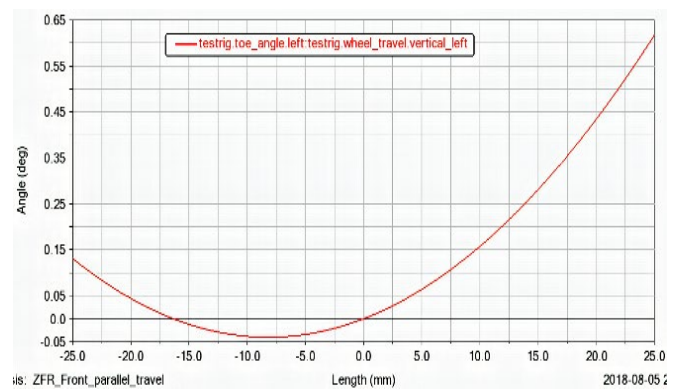
Toe change vs wheel travel
