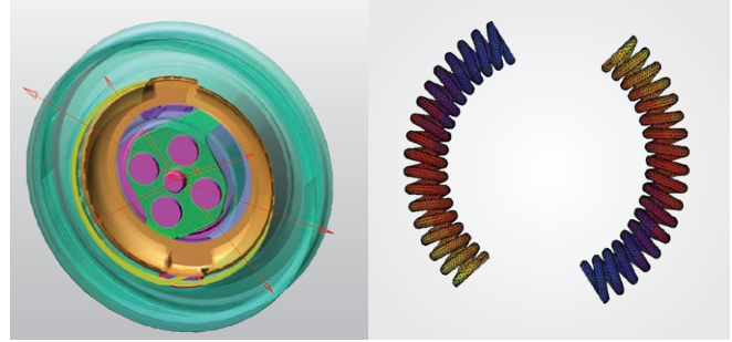
Adams Model of the center drive and Marc model of the two springs
