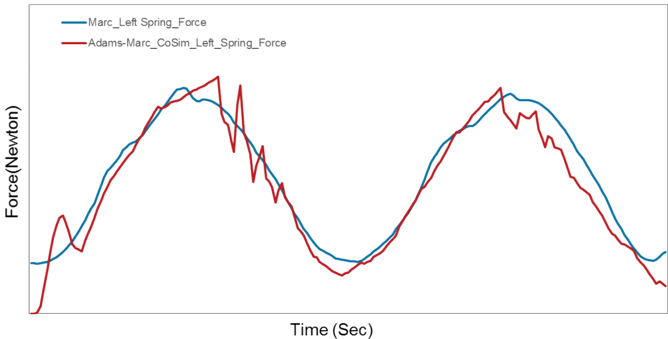
Comparison of dynamic spring load for left spring for Marc simulation vs Adams-Marc co-simulation
